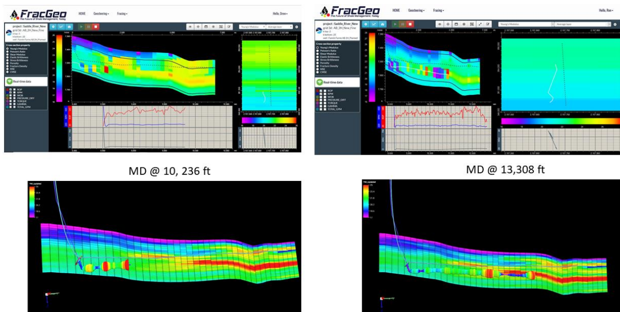
Figure 1: top windows show the GMXSteering web-based interface at two drilling depths. The interface includes the cross section along the well and the resulting updated 3D model using the derived geomechanical logs that were estimated from surface drilling data such as ROP (red curve) and RPM (blue curve). Bottom windows shows the derived Young's Modulus logs in a cross section showing the initial estimated model.
