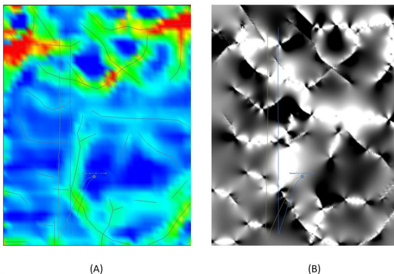
Figure 3: (A) Equivalent Fracture Model (EFM) used as input in the reservoir geomechanics that provides the (B) differential stress which provides the lateral stress gradients needed to geoengineer the stages
