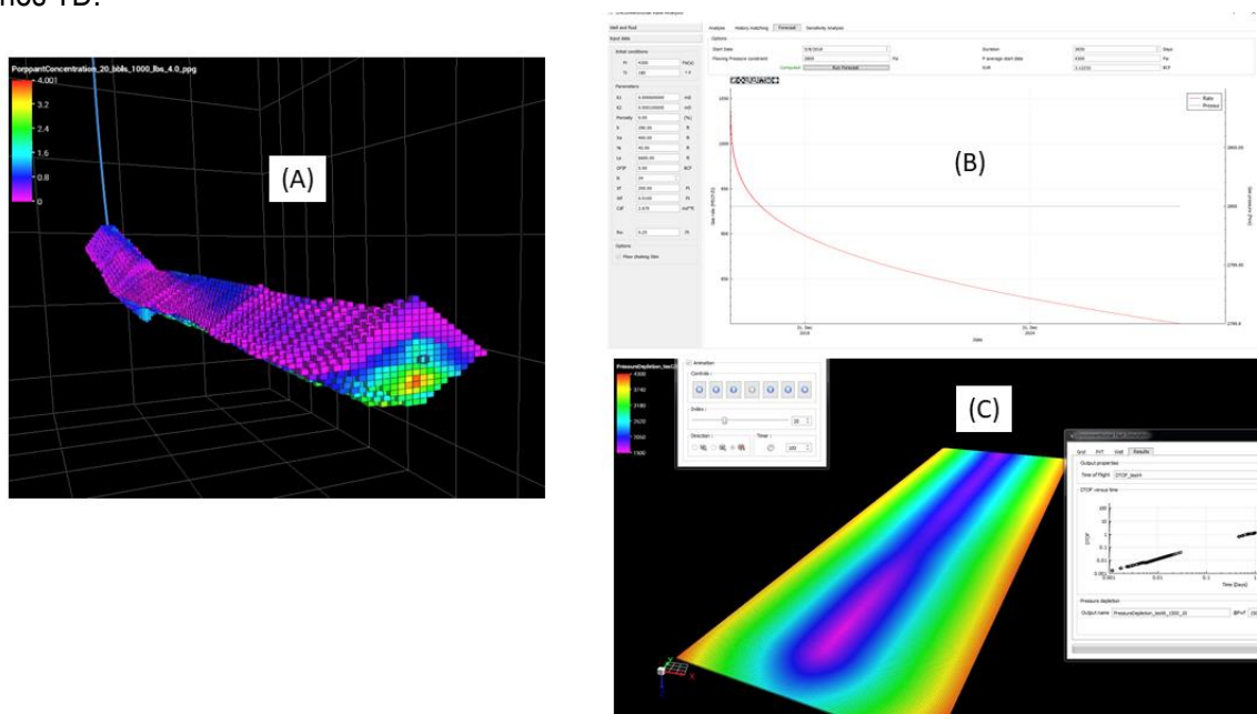
Figure 5: (A) fracture geometry along the wellbore and (B) resulting EUR and well performance estimated by using the asymmetric tr-linear model. (C) Pressure depletion around the wellbore estimated using the Fast-Marching Method (FMM) simulator
